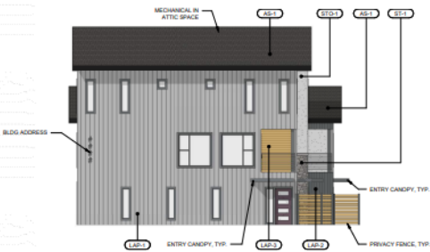
3 bldg A - street 1/8" = 1'-0"
