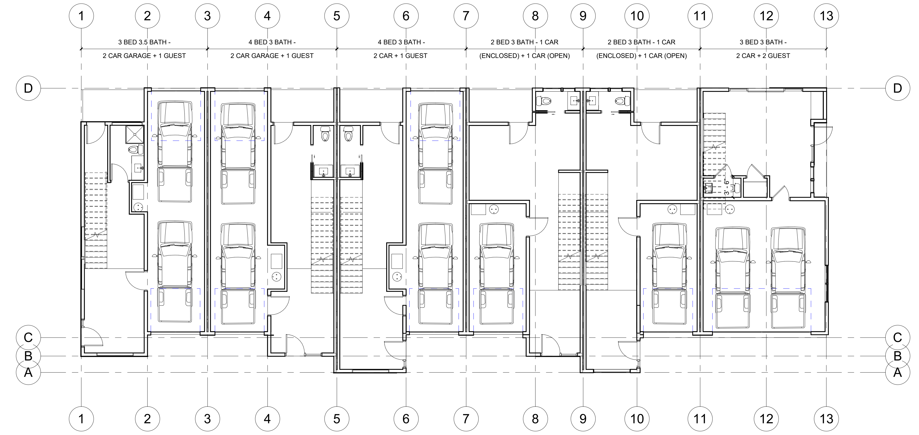
1 Level 1 1/8" = 1'-0"
