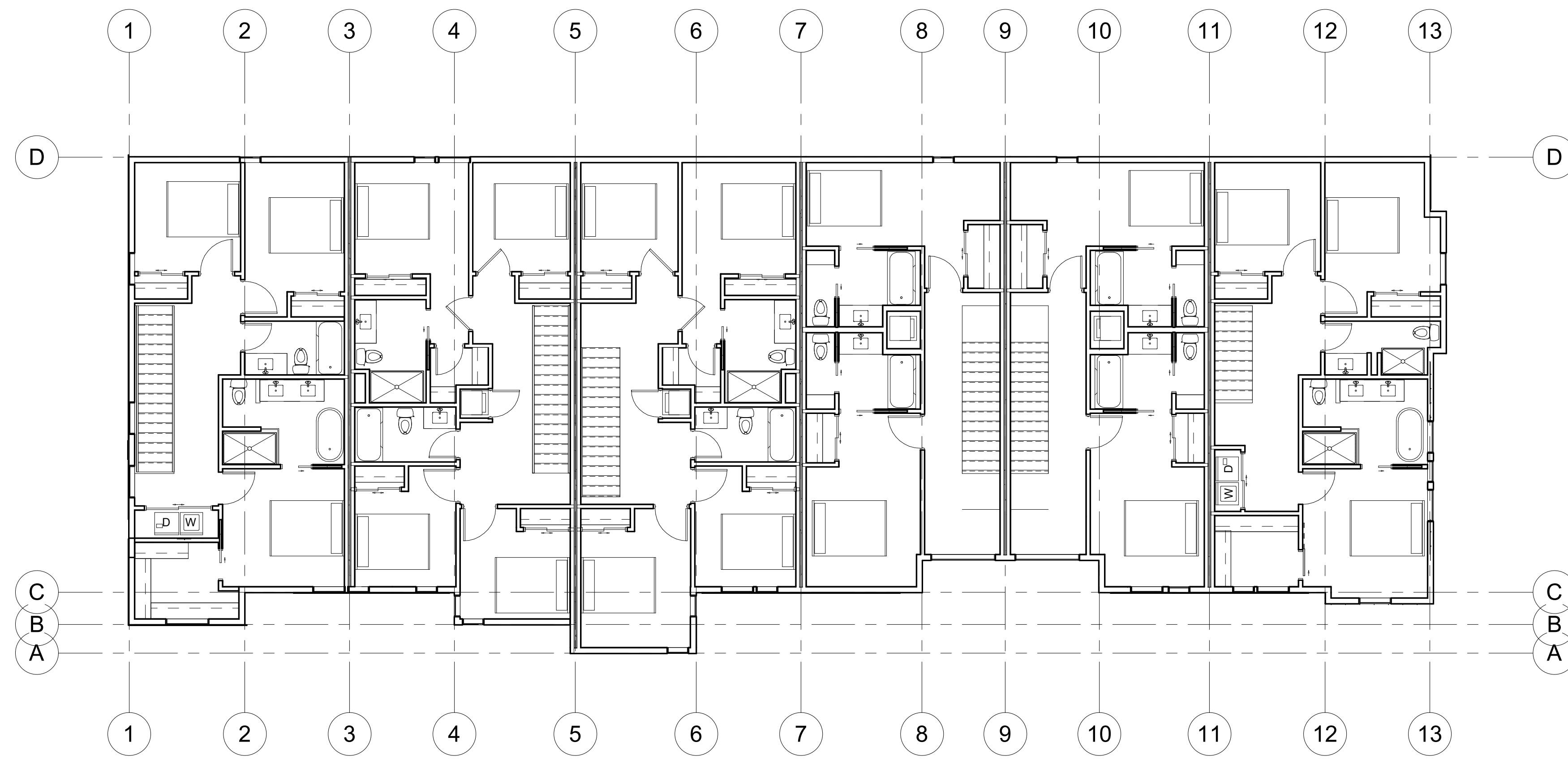
3 Level 3 1/8" = 1'-0"
